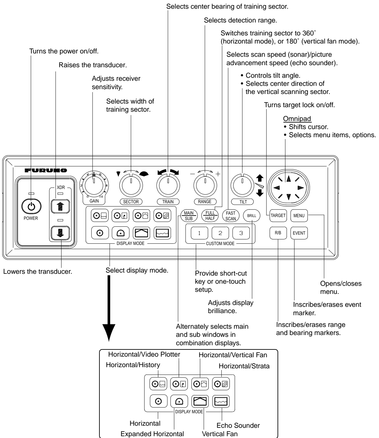
Figure 1-1 Control unit
